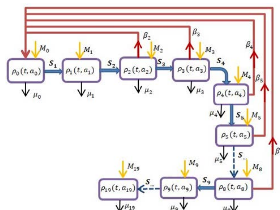
Figure 2 Model Flow chart showing interaction of population clusters. The population densities denoted by \rho_0(t, a_0), \rho_1(t, a_1), \dots, \rho_{19}(t, a_{19}) , death rates is given by \mu_0, \mu_1, \dots, \mu_{19} , migration rates into the cluster is M_0, M_1, M_2, \dots, M_{19} transition rates S_1, S_2, \dots, S_{19} , birth rates \beta_2, \beta_3, \dots, \beta_8 .
