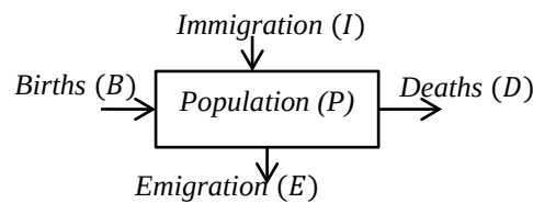
Figure 1: Compartmental model showing changes in population compartment
