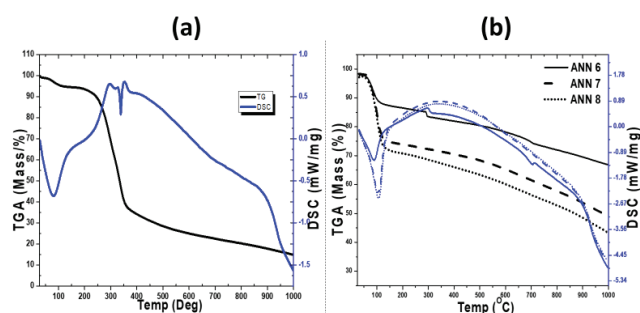
Figure 4: TGA/DSC profile (a) Zea mays cobs and (b) activated carbon ANN6, ANN7 and ANN8 sample materials.
