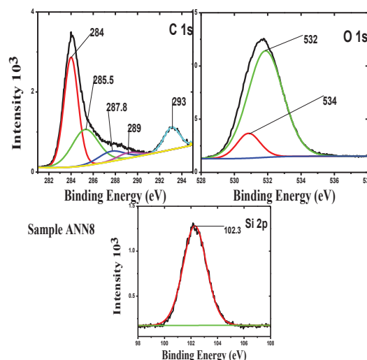
Figure 3: XPS deconvoluted spectra for ANN8 activated carbon sample.
