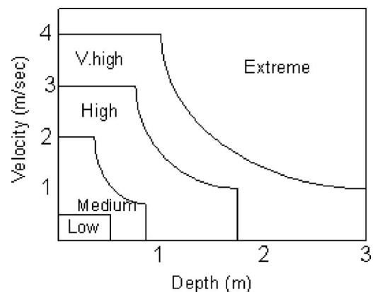
Figure 11. Flood hazard categories with respect to calculated velocities and depths.
