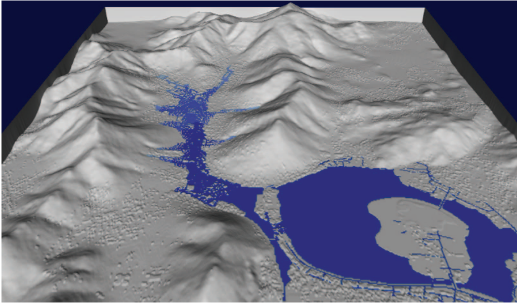
Figure 2. 3-dimensional view of the water surface simulated using a 1D-2D coupled model (St Maarten). The coupling in this example involves channel flows generated by a 1D model superimposed on the flood plain identified by a digital terrain model (DTM) of the 2D ground surface. In the DTM, elevation levels of all buildings are raised by 5m and all roads are lowered by 0.25m in order to represent actual physical conditions.
