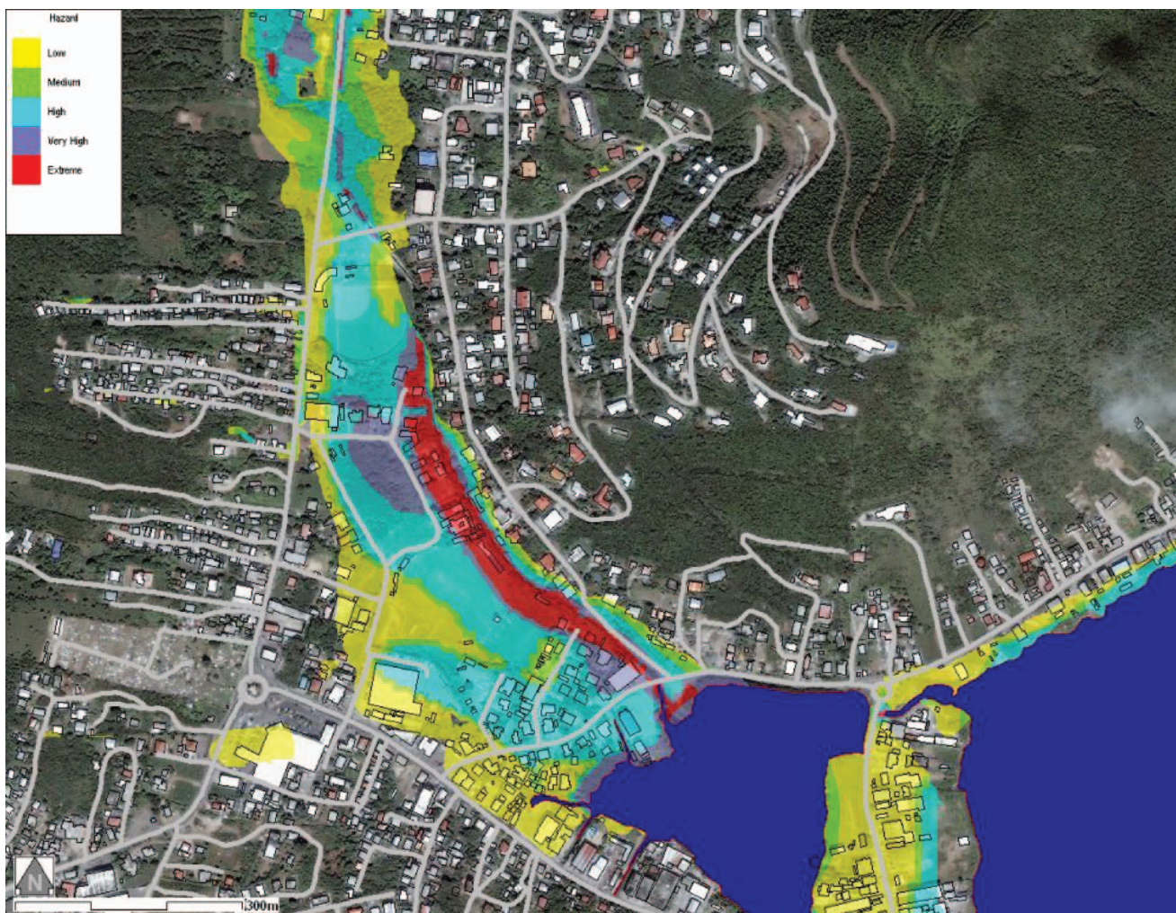
Figure 1. An example of a road network and modelled flood hazard data presented in a GIS environment (UNESCO-IHE 2007).
