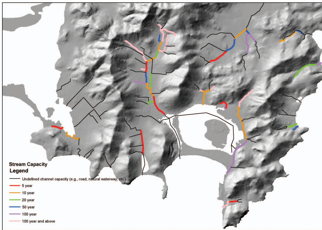
Figure 8. A GIS map of all modelled channels and their corresponding capacities.
