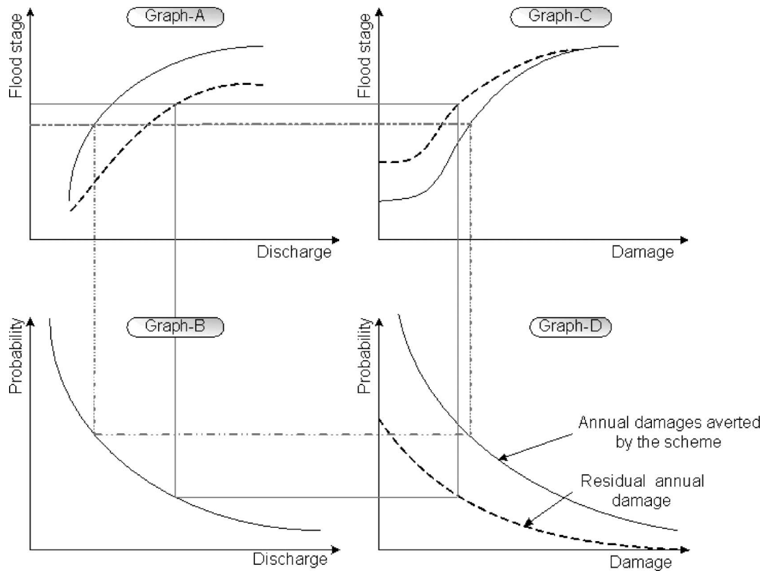
Figure 6. Annual flood damage assessment (Penning-Rowsell and Chatterton 1977). The graphs show damage values before (solid line) and after (dashed line) rehabilitation.
