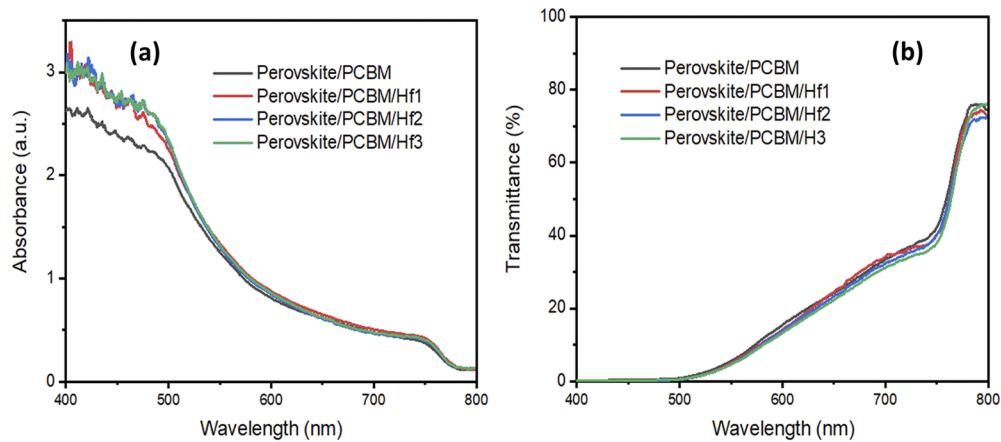
FIG. 2. (a) Absorbance and (b) transmittance spectra of various concentrations of the Hfaca layer and the control.
