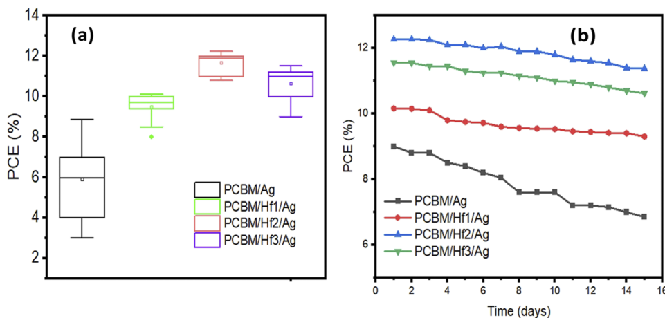
FIG. 4. (a) Statistical performance of all the devices fabricated, (b) stability of devices fabricated with the PCBM/Ag control device and devices fabricated with different concentrations of Hfaca.
