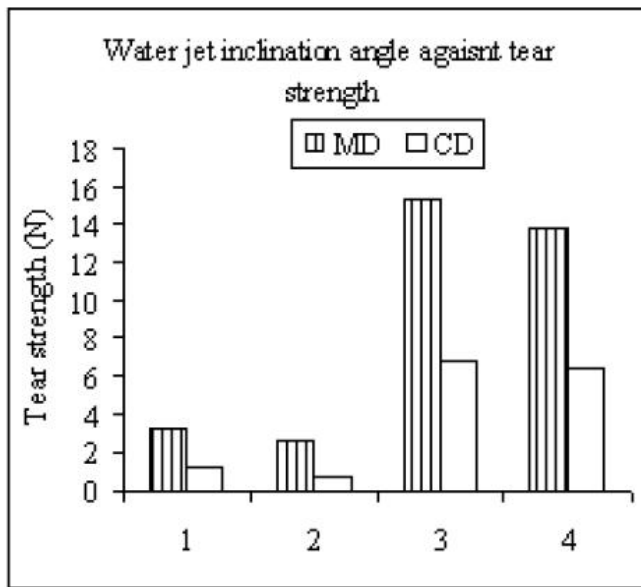
(a) Fabrics (PA6/PET), 60 gsm
