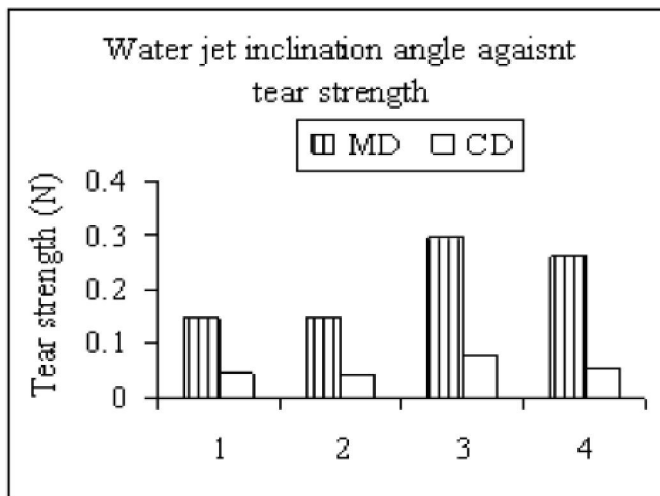
(a) Fabrics (PET/COPET), 60 gsm
