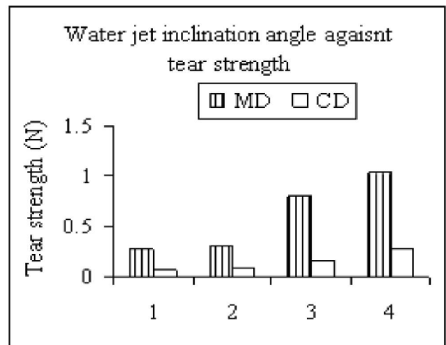
(b) Fabrics (PET/COPET), 100 gsm
