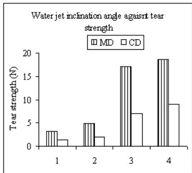
(b) Fabrics (PA6/PET), 100 gsm
