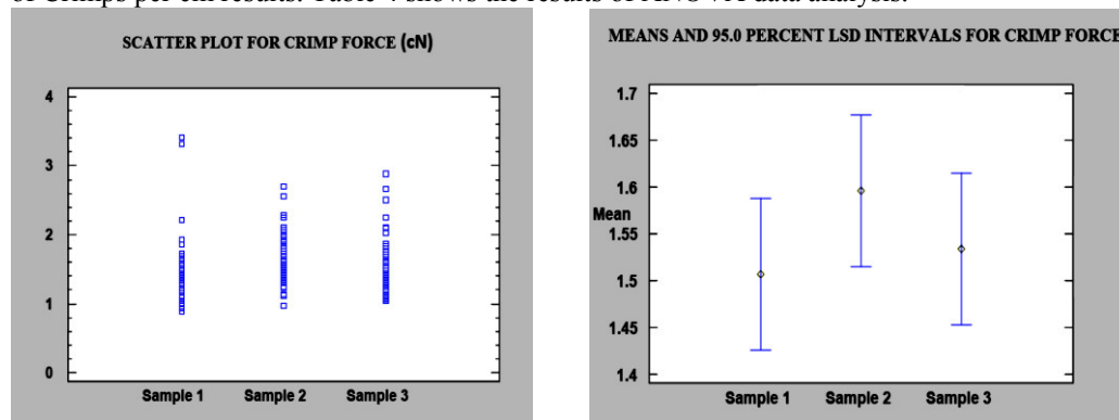
Figure 5: Crimp Force results
