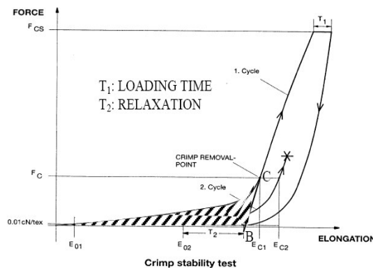
Figure 2: Force-Extension Curve in the Crimp Stability Test (Evans& Montgomery, 1953).
