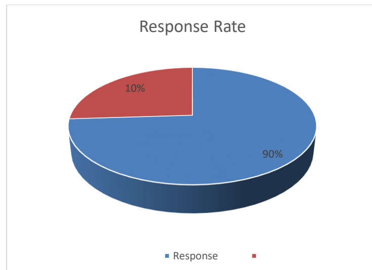
Figure 4.1: Response Rate
