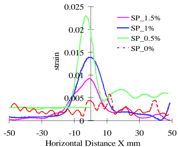
(c) Ultimate deformation profile across centre face
