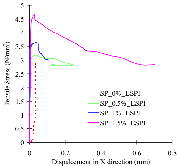
(b) Tensile Stress-Displacement
