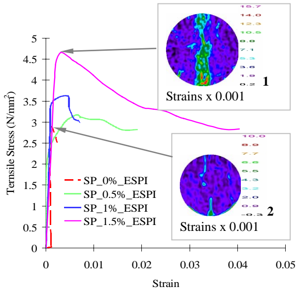
(a) Tensile strength and full field ultimate deformation pattern
