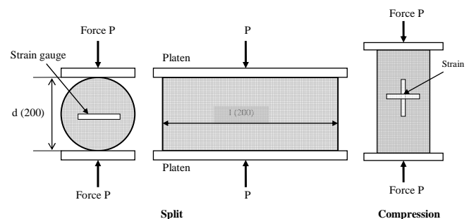
(b) Split and Compression
