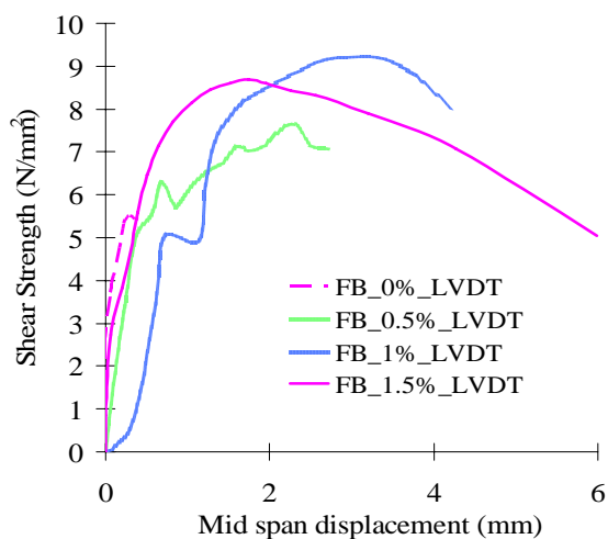
(b) LVDT Measurement
