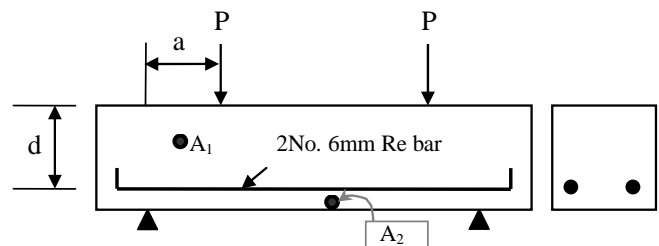
(a) Flexure (Indirect shear)
