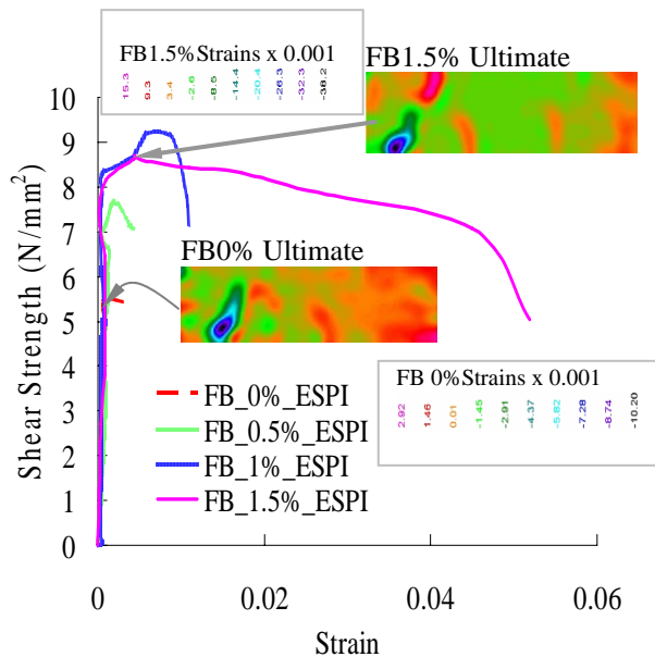
Fig 7 Shear strength-strain relationship and deformation Behavior
