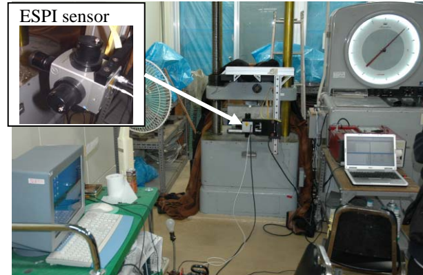
Fig.2 Optical and Normal test set up
