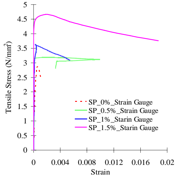
Fig. 5 Conventional Stress-strain measurements
