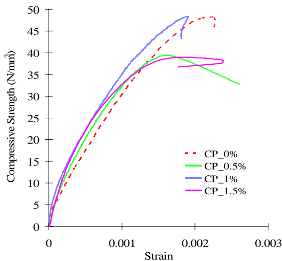
Fig.6 Compression strength
