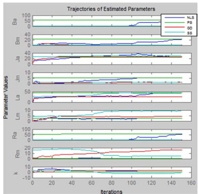
Figure 11. Simulation Trajectories.
