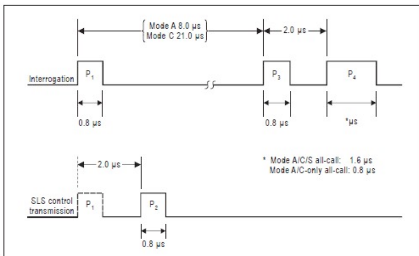
FIGURE 1-12: INTERMO DE INTERROGATION PULSE SEQUENCE
