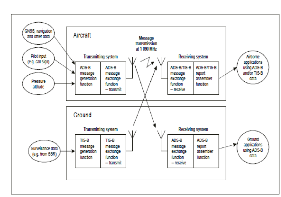
1.1.FIGURE1-1: ADS-B/TIS-B SYSTEM FUNCTIONAL MODE
