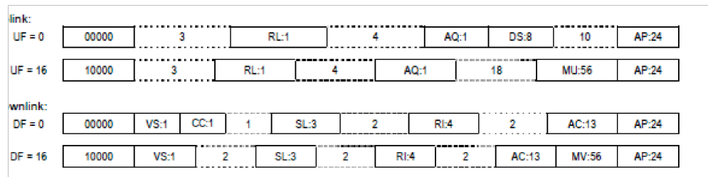
Figure 6-1: Surveillance and Communication formats used by ACAS
