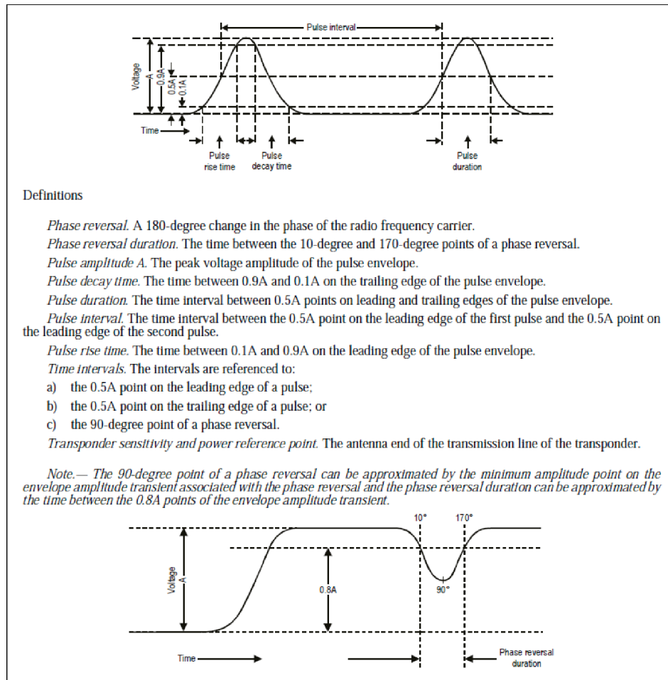
Figure 3-1. Definitions of secondary surveillance radar waveform shapes, intervals and the reference point for sensitivity and power
