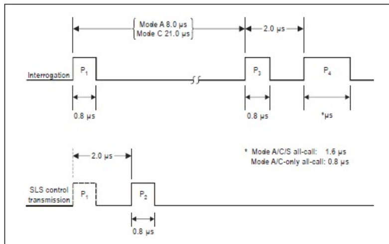
Figure 3-3. Intermode interrogation pulse sequence
