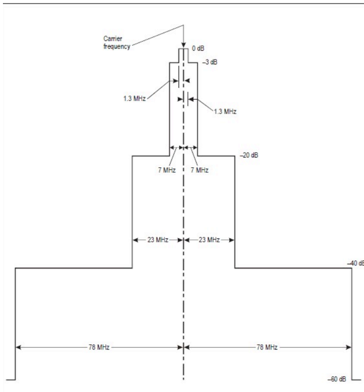
FIGURE 1-14: REQUIRED SPECTRUM LIMITS FOR TRANSPONDER TRANSMITTER-
