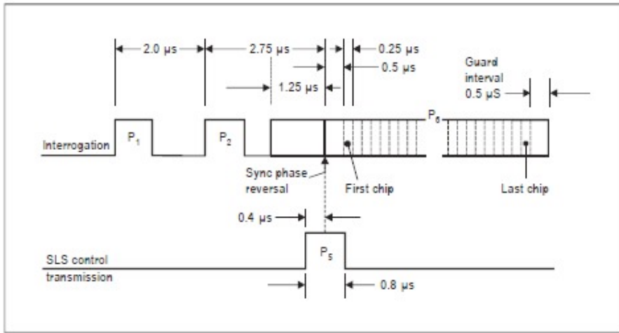
Figure 3-4. Mode S interrogation pulse sequence
