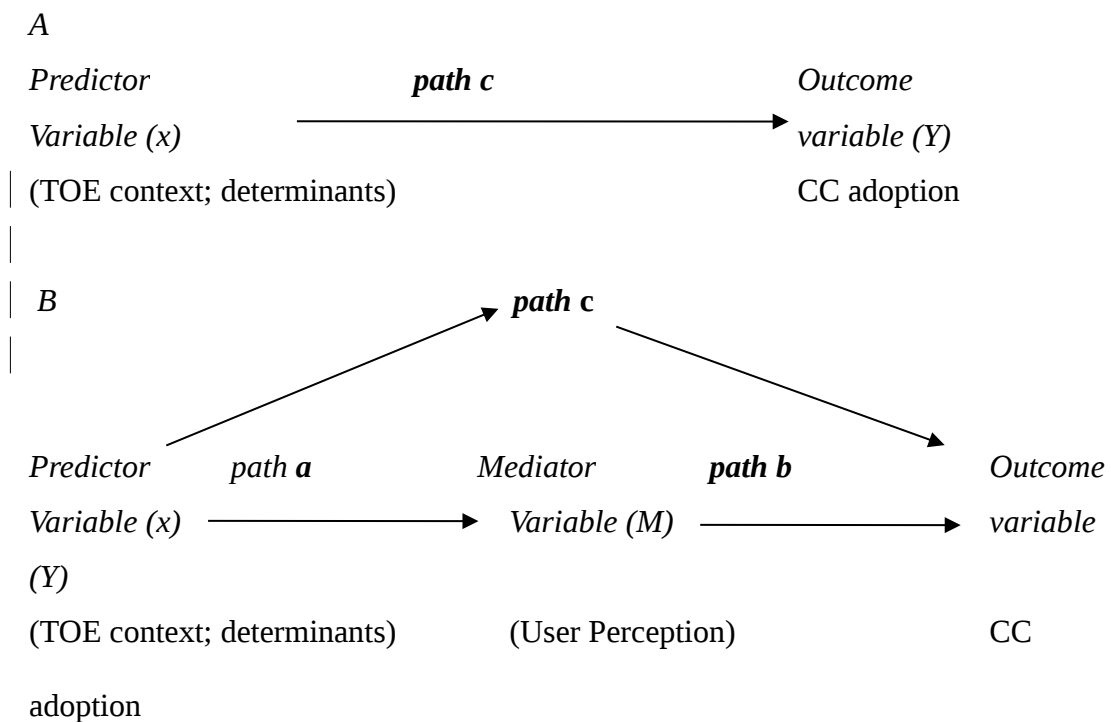
Figure 3.1: Diagram of Path in Mediation Models
